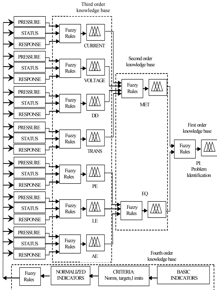
Fig. 2.- Configuration of the fuzzy expert system
